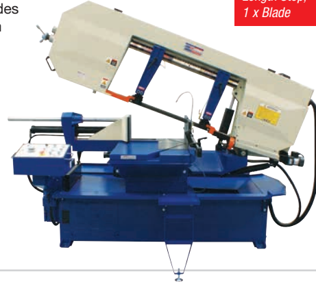
Hydraulic Full Length Vice
