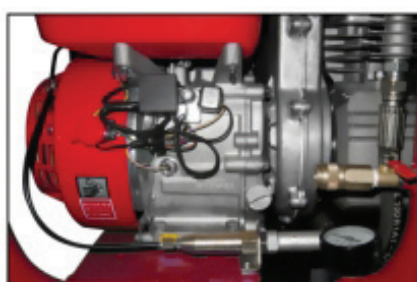
Pilot Valve & Cold Start Valve
