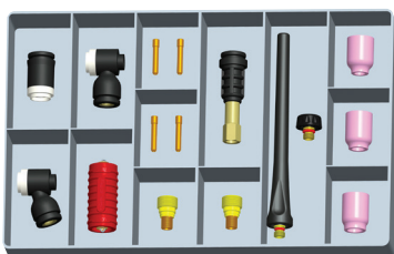
9-Series Torch Contractors Kit RNK-9-150
