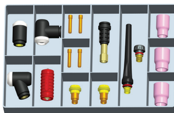
17-Series Torch Contractors Kit RNK-17-150
